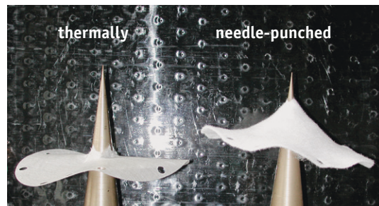
Figure 6 Typical behaviour of 200g/m 2 needle-punched and thermally bonded nonwovens in the cone drop test (simulation of a puncture load)
