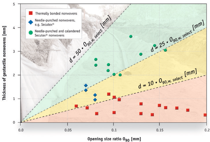
Figure 8 Recommended opening size and thickness correlation for a filter geotextile (DVKW, Vol. 221/1992)
