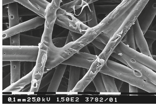
Figure 4 Thermally bonded nonwoven [1]
