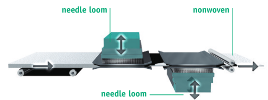
Figure 2 Needle-punched nonwoven process
