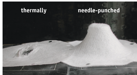
Figure 5 Typical behaviour of 200g/m 2 needle-punched and thermally bonded nonwovens in the plunger puncture test (simulation of a stone puncture)
