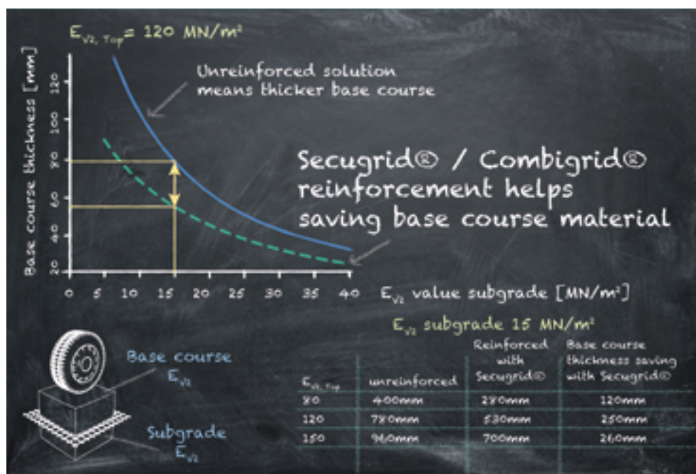
Figure 20: Comparison between non-reinforced and Secugrid® or Combigrd® reinforced sub-base or base course
