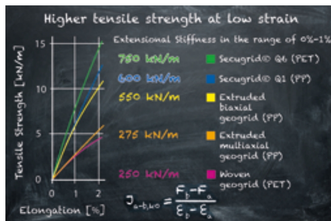
Figure 8: Exemplary stress-strain curves for Secugrid®, Combigrig® and other geogrids in the strain range of between 0% to 2% at comparable ultimate tensile strength levels
