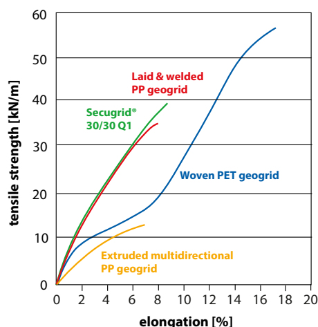
Figure 28: Stress-strain curves of 4 tested geogrids in Montana field trial (Phase II, 2014)
