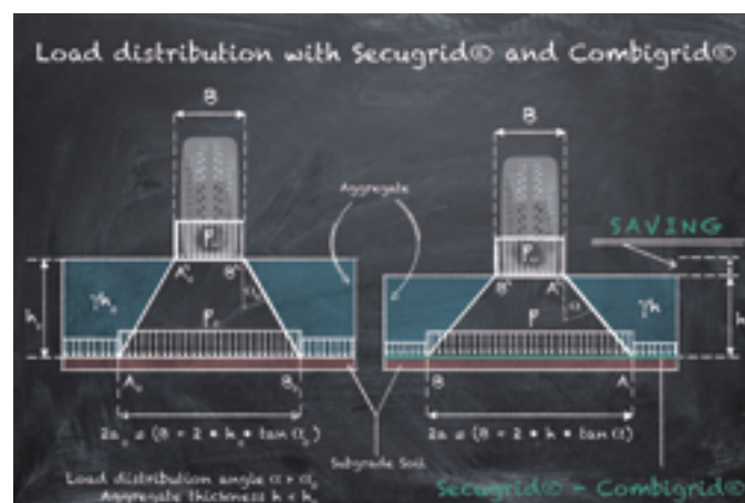
Figure 1: Saving of granular material in the base course by using Secugrid® and Combigrd® stabilisation and reinforcement products
