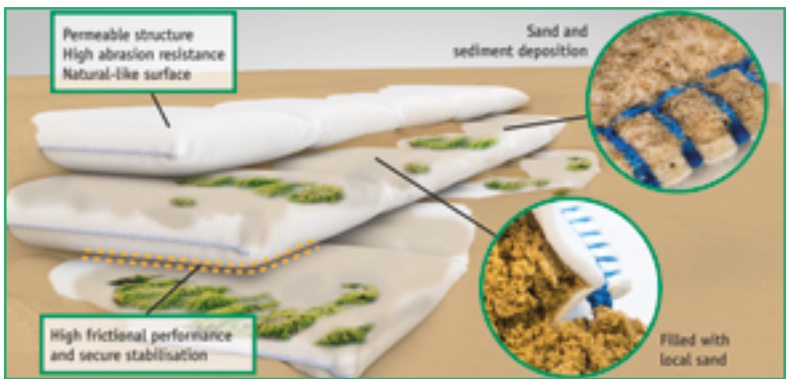
Figure 4: Advantages of Secutex® Soft Rock GSCs
