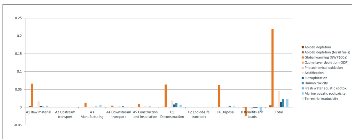
Fig. 6.2 Environmental external costs of the different life cycle stages (A1 – A5, C1 – C4, D, and Total, excluding D) of the manufacture and disposal of 1 sqm average Secumat®
