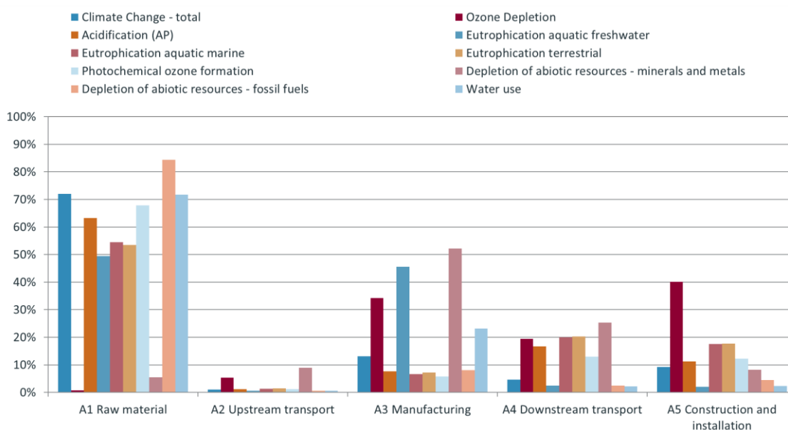
Fig. 4.1 Relative contribution of the different life cycle stages (A1 – A5) to the total impact of the product and construction process stage A of Secumat®
