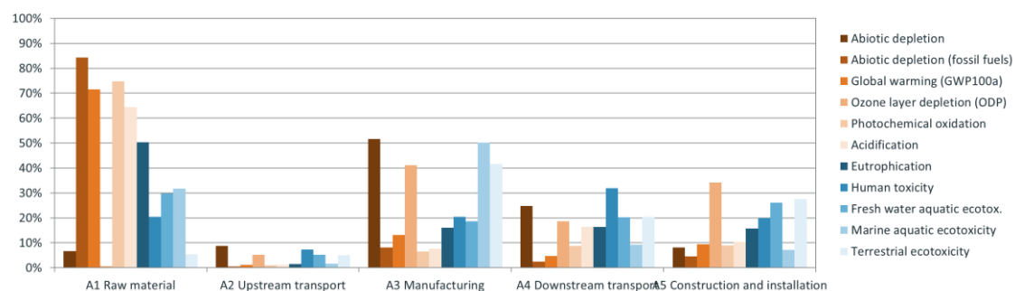
Fig. 6.1 Relative contribution of the different life cycle stages (A1 – A5) to the total environmental impacts of the product and construction process stage A of Secumat®
