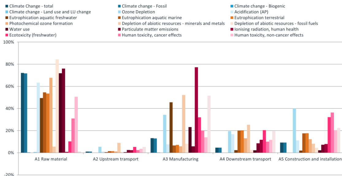
Fig. 5.1 Relative contribution of the different life cycle stages (A1 – A5) to the total impact of the product and construction process stage A of Secumat®
