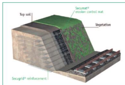
Figure 4 Secumat® as spray-on vegetation solution
