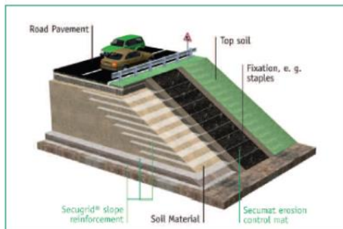
Figure 2 Secumat® as erosion control for a reinforced slope
