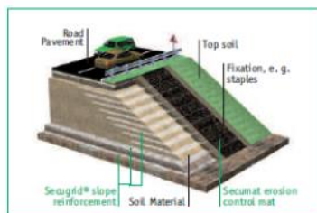
Figure 2 Secugrid® reinforced slope with 45° inclination
