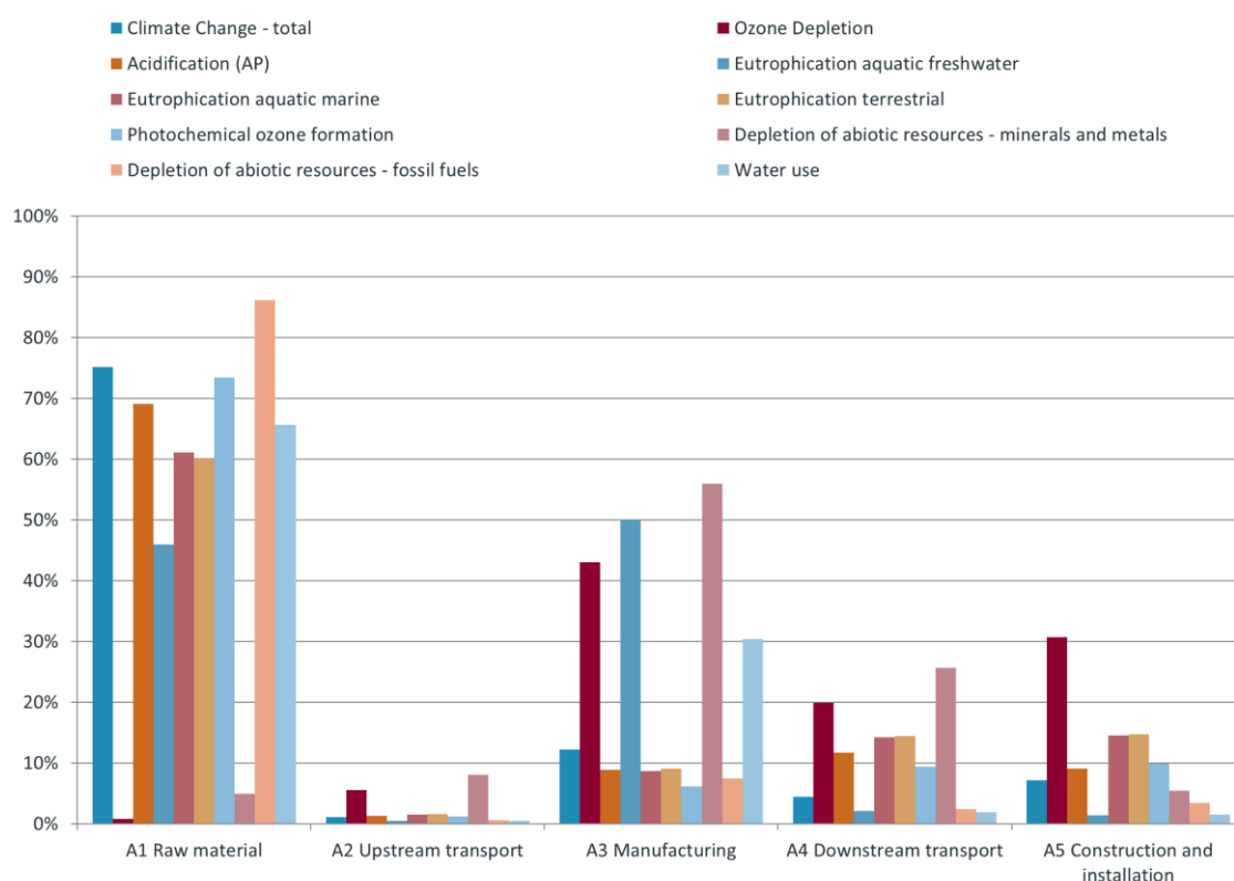
Fig. 4.1 Relative contribution of the different life cycle stages (A1 – A5) to the total impact of the product and construction process stage A of the average geosynthetic drainage element Secudrain®
