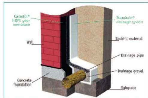
Figure 3 Secudrain® - Drainage of an underground structure
