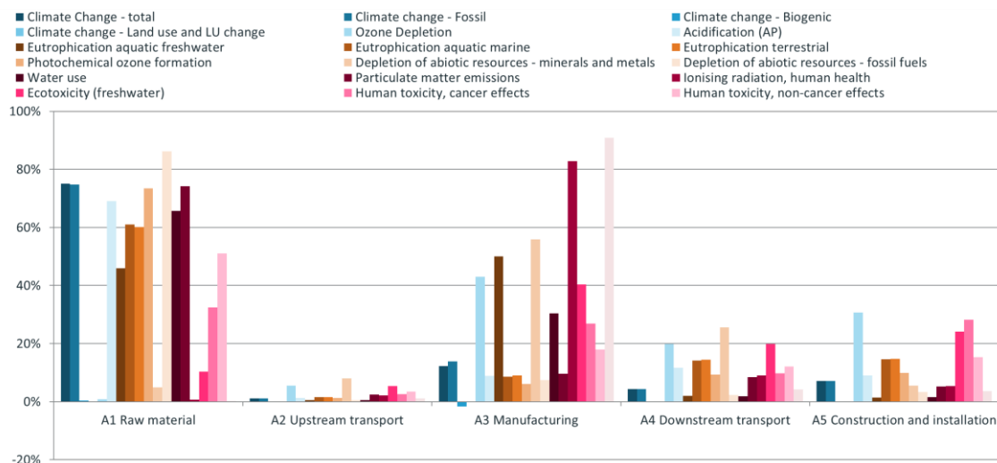
Fig. 5.1 Relative contribution of the different life cycle stages (A1 – A5) to the total impact of the product and construction process stage A of Secudrain®
