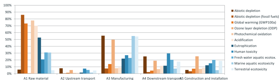
Fig. 6.1 Relative contribution of the different life cycle stages (A1 – A5) to the total environmental impacts of the product and construction process stage A of Secudrain®
