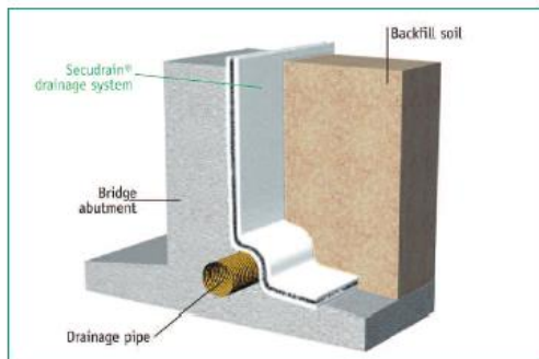
Figure 2 Secudrain® - Drainage of a bridge abutment
