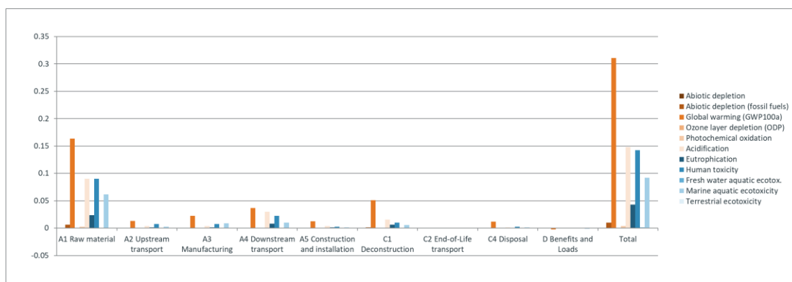
Fig. 6.2: Environmental external costs of the different life cycle stages (A1 – A5, C1 – C4, D, and Total, excluding D) of the manufacture and disposal of 1 m 2 average Bentofix®
