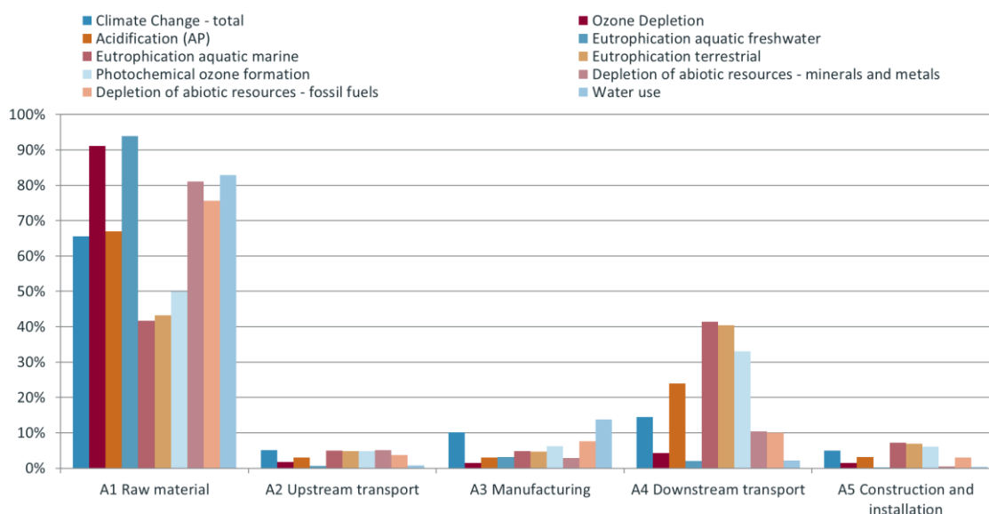
Fig. 4.1 Relative contribution of the different life cycle stages (A1 – A5) to the total impact of the product and construction process stage A of Bentofix ®
