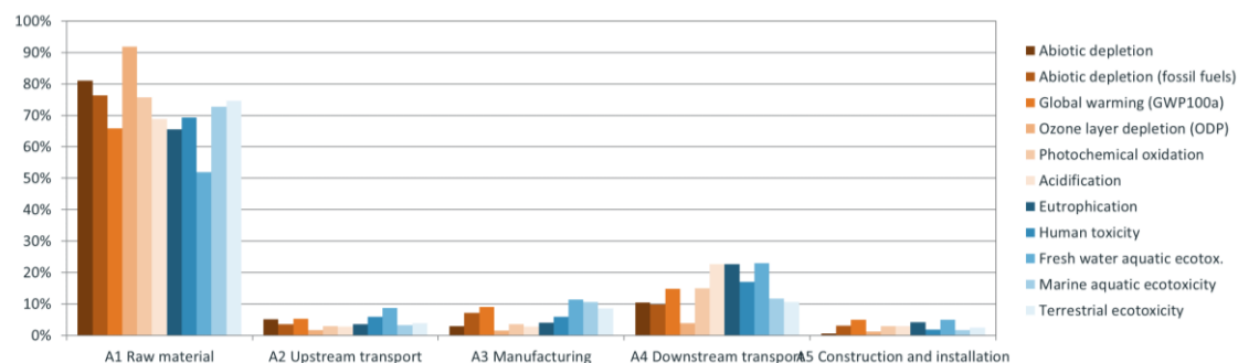
Fig. 6.1: Relative contribution of the different life cycle stages (A1 – A5) to the total environmental impacts of the product and construction process stage A of Bentofix®
