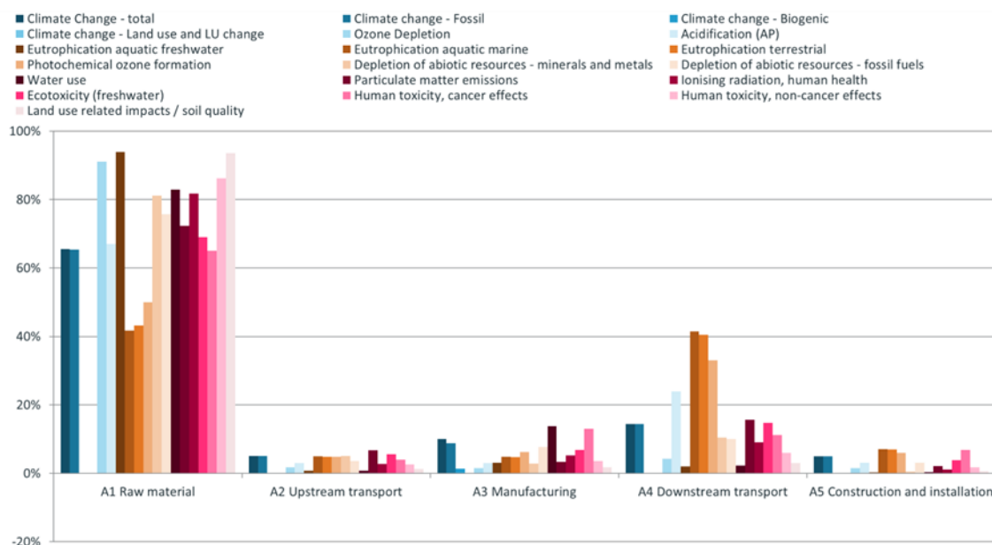
Fig. 5.1 Relative contribution of the different life cycle stages (A1 – A5) to the total impact of the product and construction process stage A of Bentofix®
