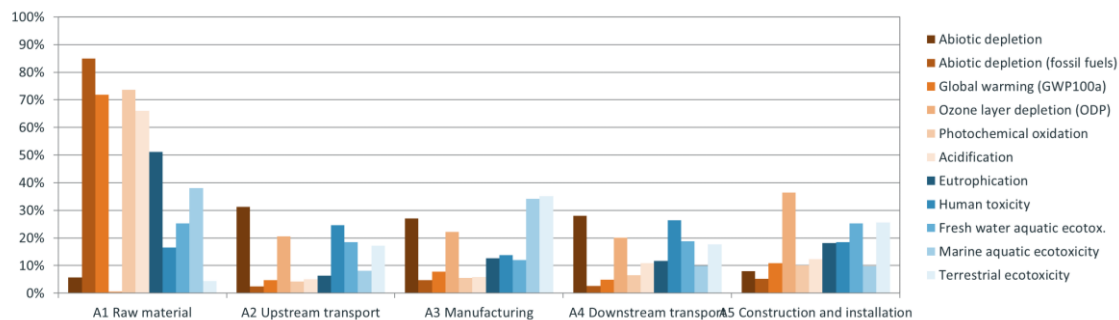
Fig. 6.1 Relative contribution of the different life cycle stages (A1 – A5) to the total environmental impacts of the product and construction process stage A of Secutex®
