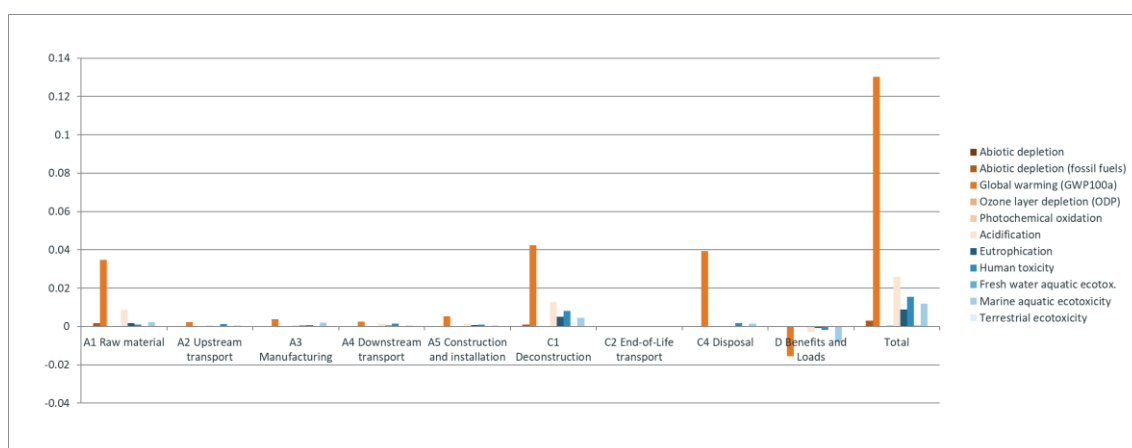
Fig. 6.2 Environmental external costs of the different life cycle stages (A1 – A5, C1 – C4, D, and Total, excluding D) of the manufacture and disposal of 1 sqm average Secutex®
