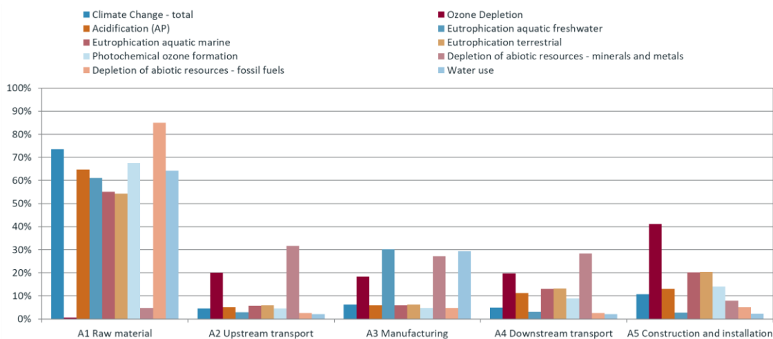
Fig. 4.1 Relative contribution of the different life cycle stages (A1 – A5) to the total impact of the product and construction process stage A of Secutex®
