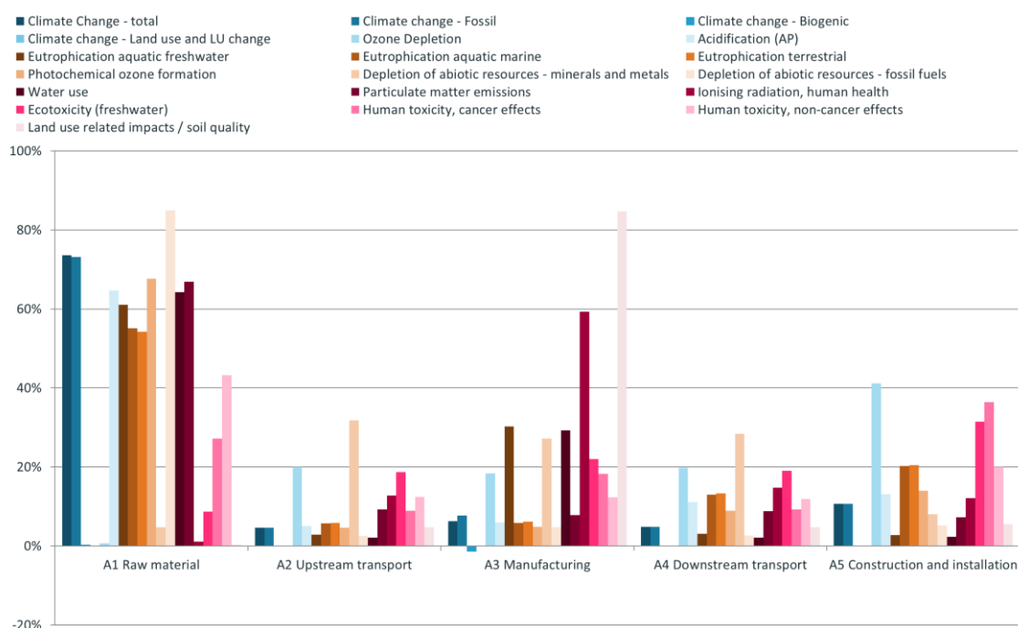
Fig. 5.1 Relative contribution of the different life cycle stages (A1 – A5) to the total impact of the product and construction process stage A of Secutex ®
