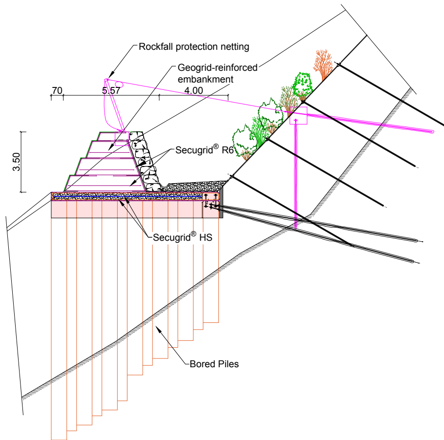
Fig. 1: Cross section protection embankment Laugneri II
